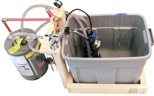
Figure 5: Test measurement setup. A pump, point-of-use hot water heater, shower head, and tub simulate a shower, allowing for small-scale experiments with controlled temperatures.
