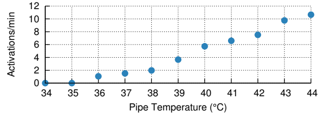
Figure 1: Activation rate of Thermes at a range of pipe temperatures in 23°C ambient conditions. As the temperature difference between each side of the Peltier module increases, so too does the average rate of activations over the first five minutes of harvesting.
